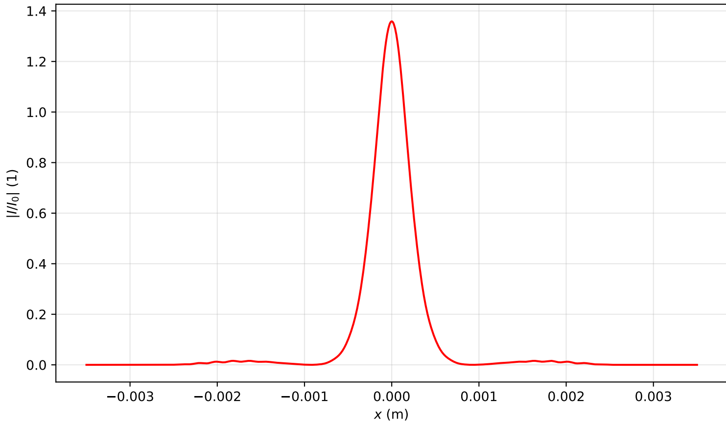
Intensity profile I(x, y = 0, z = 1.274)/I_0 , P_{in}=1.0P_{cr} , artificial time
